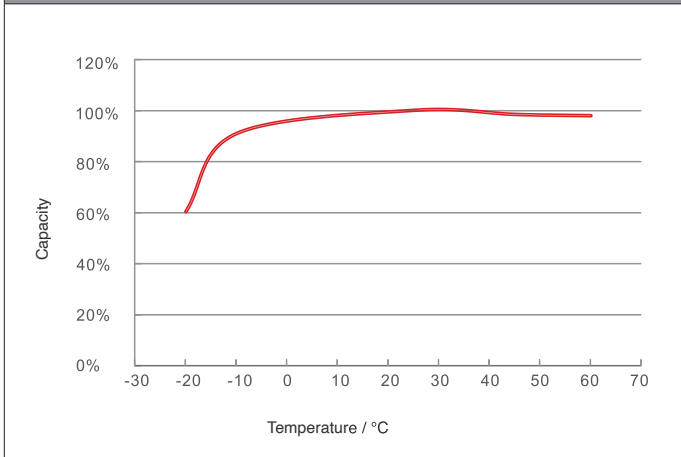
Different Temperature Capacity Curve
