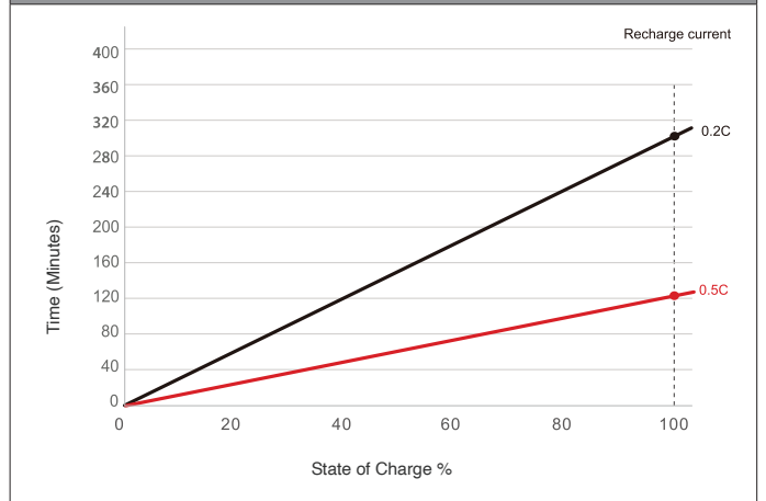
Typical Charge Time Curve
