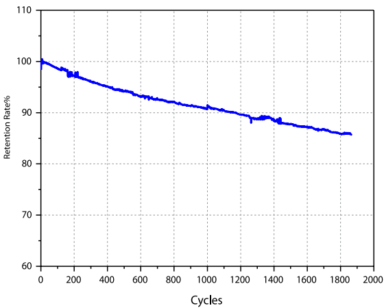
Cycles & Capacity Retention @ 0.2C
